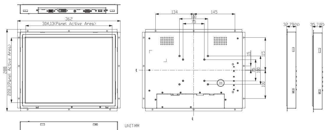
Figure 2.1 IDS-3115 Series Dimensions
