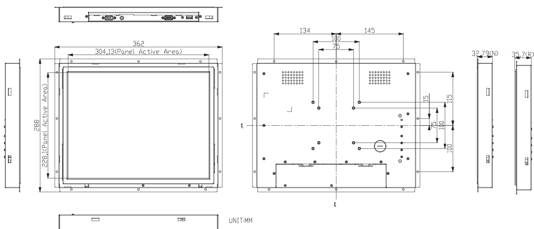
Figure 2.2 IDS-3115E Series Dimensions
