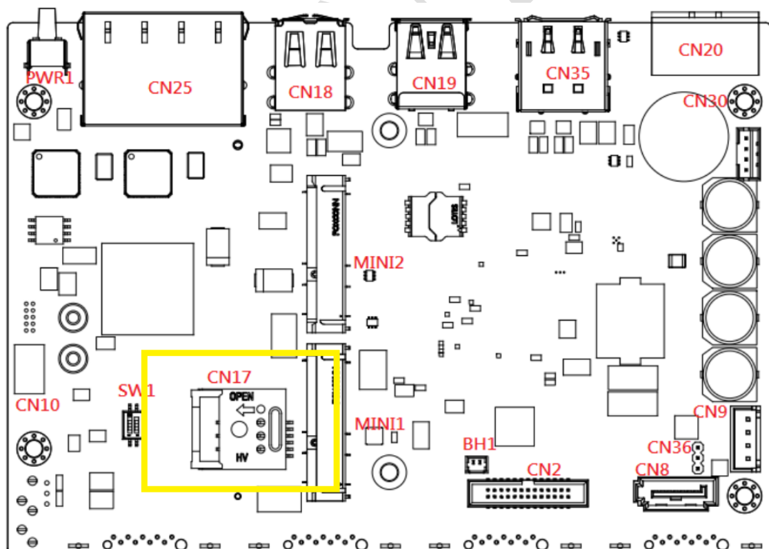
Figure A.1 Connector & Switch Locations on MB(Top)
