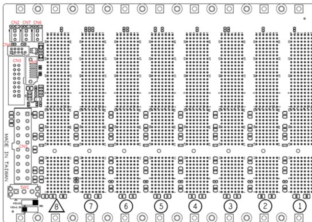
Figure 3.2 MIB-3109P7 Rear View
