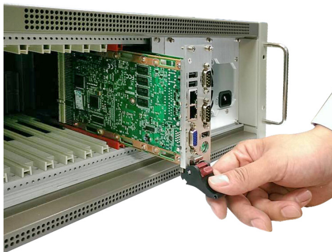
Figure 2.10 Inserting a Peripheral Card
