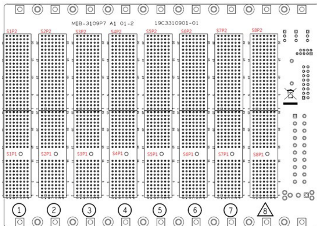
Figure 3.1 MIB-3109P7 Front View
