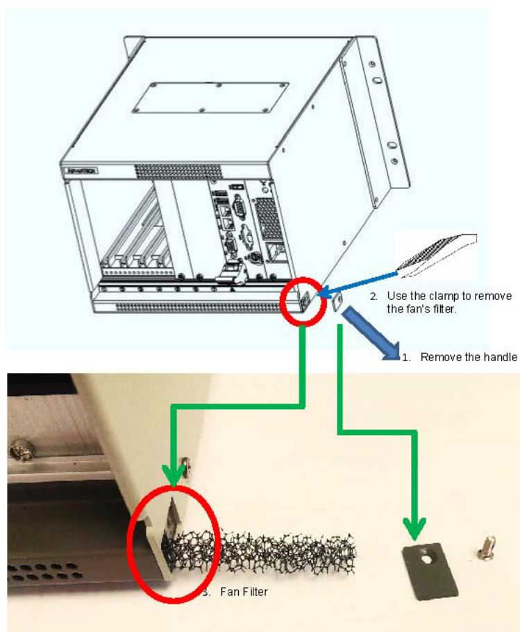
Figure 2.8 Fan Filter
