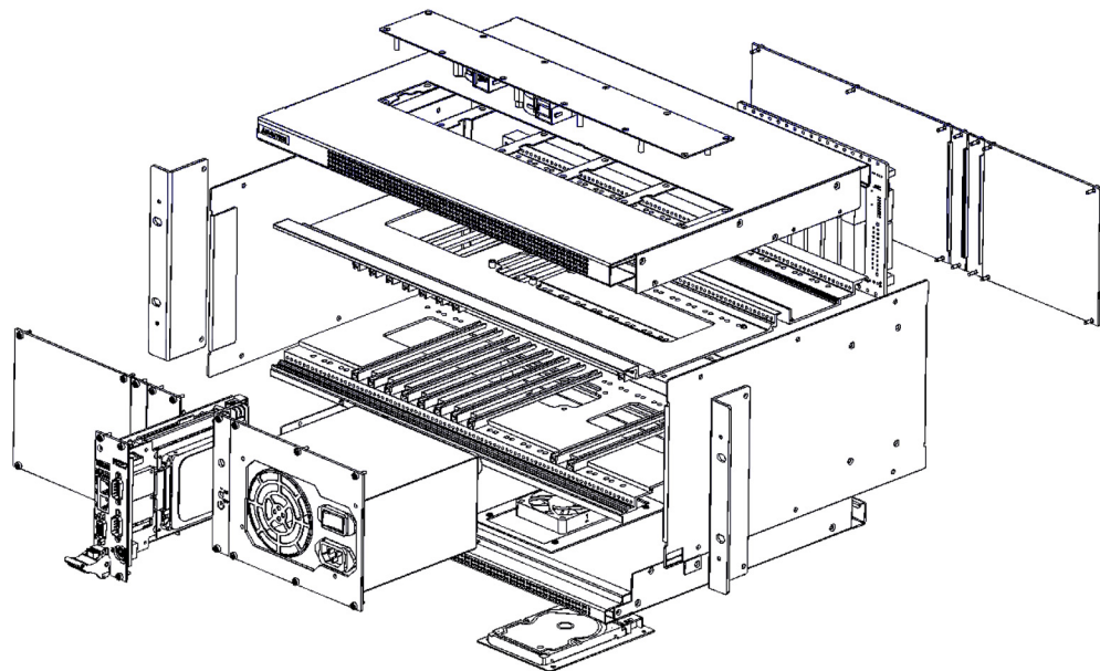
Figure 1.2 Exploded View
